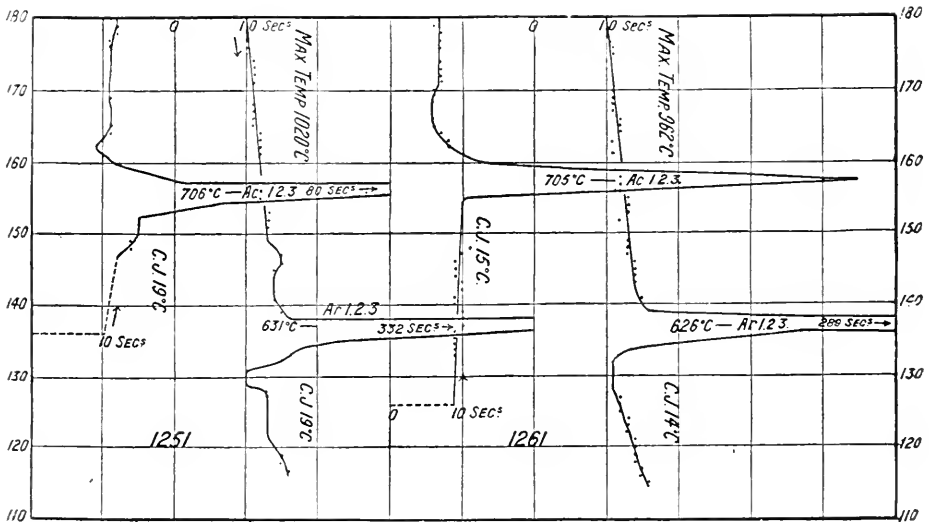
Heating and Cooling Curves of 3 per cent. Nickel Steels, with 0.74 and 0.91 per cent. of Carbon respectively
